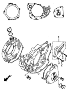
BLOCK No. E-3 CRANKCASE COVER (FIG.6/9900B-68068-010)
