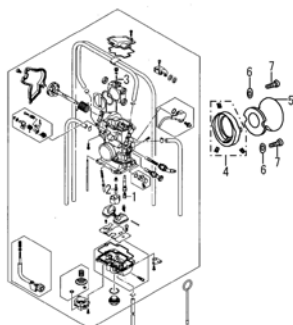
BLOCK No. E-5 CARBURETOR (FIG.10/9900B-68068-010)
