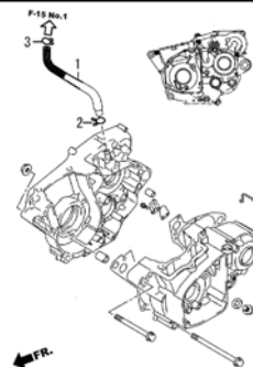
BLOCK No. E-2 CRANKCASE (FIG.5/9900B-68068-010)
