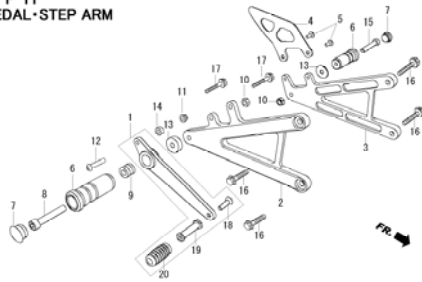
BLOCK No. F-11 BRAKE PEDAL-STEP ARM
