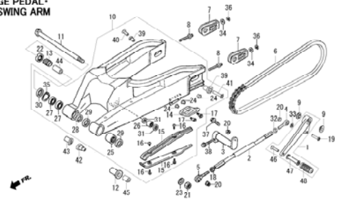
BLOCK No. F-12 CHANGE PEDAL- REAR SWING ARM
