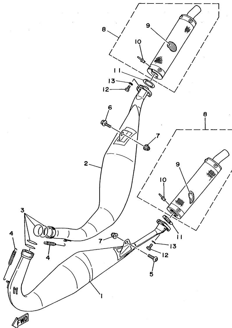
FIG. 9 EXHAUST
